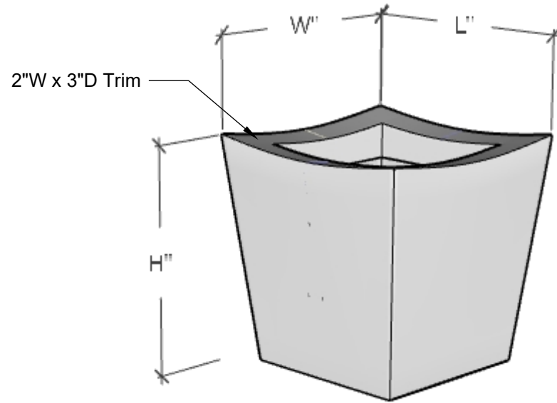
PERSPECTIVE VIEW
